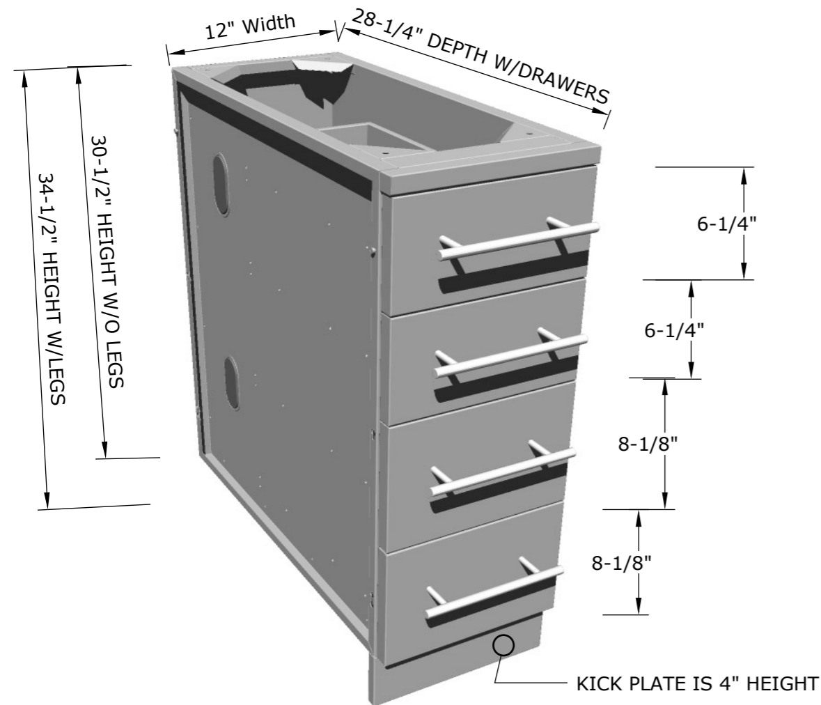
ISO VIEW
