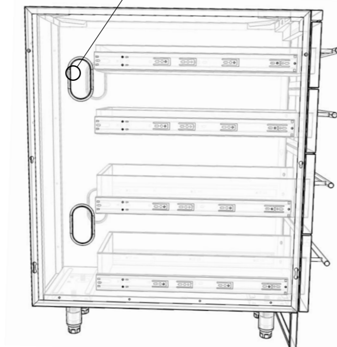
UTILITY ACCESS PORTS W/COVER
