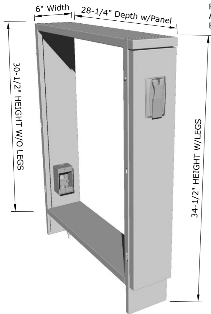
ISO VIEW
